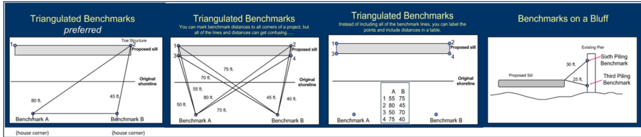
Figure 9: Benchmark Examples
