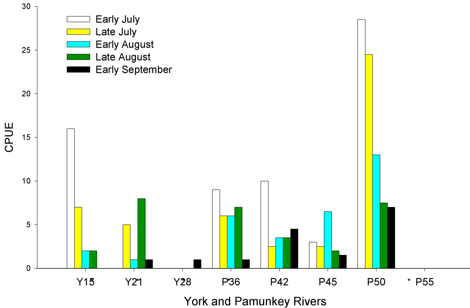
Figure 7. Catch of young-of-year striped bass by station in the York and Pamunkey rivers in 2010. Index station catch represents an average of two hauls; auxiliary station (starred) catch represents one haul. No sampling occurred at Y21 during early July or at P55 during late August and early September.
